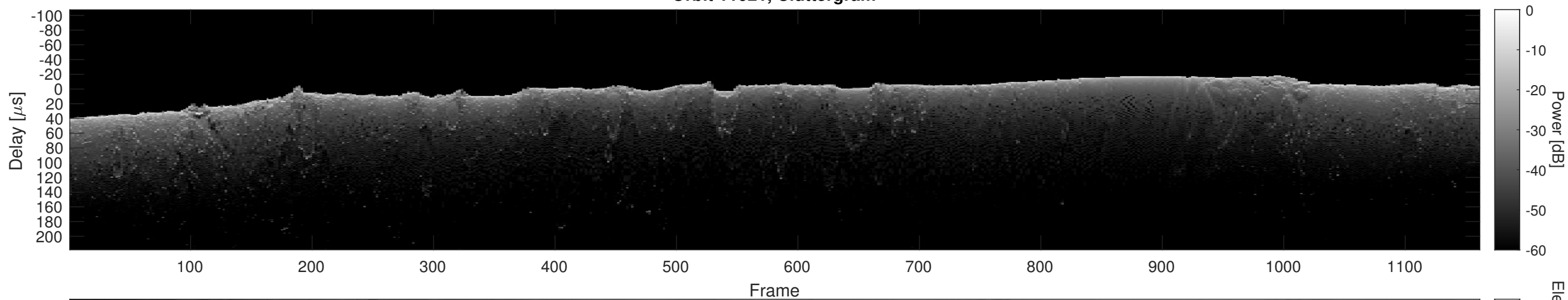
Orbit 11021, Cluttergram
