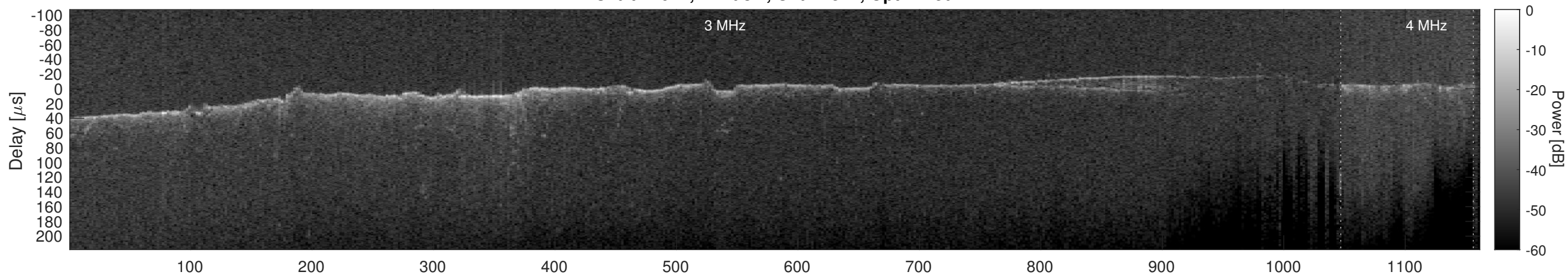
Orbit 11021, Cluttergram
