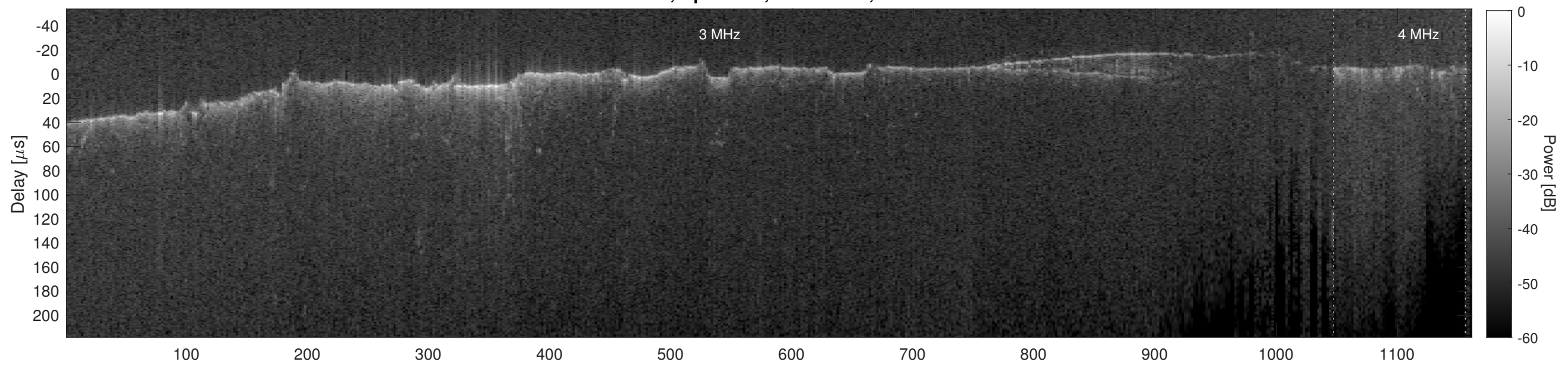
Orbit 11021, Cluttergram
