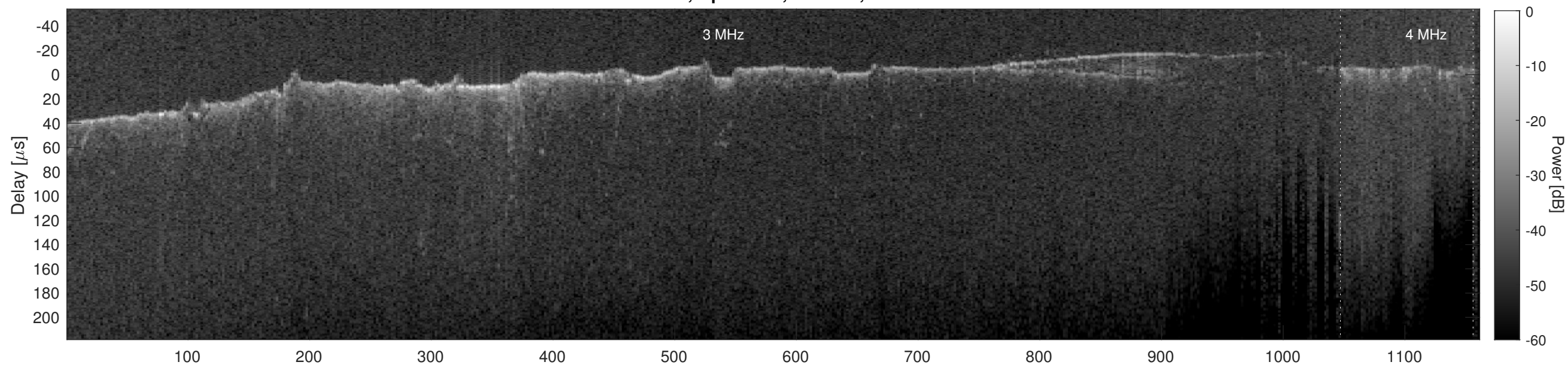
Orbit 11021, Cluttergram
