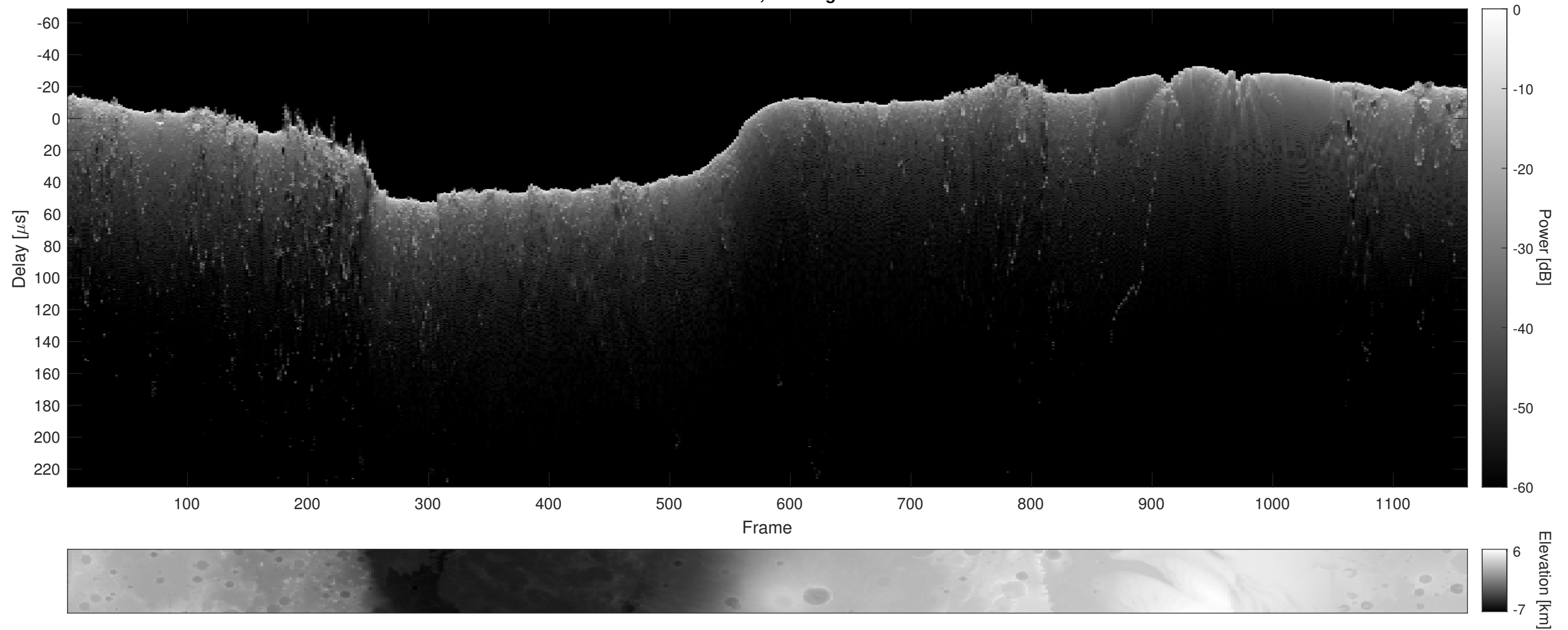
Orbit 11022, Cluttergram
