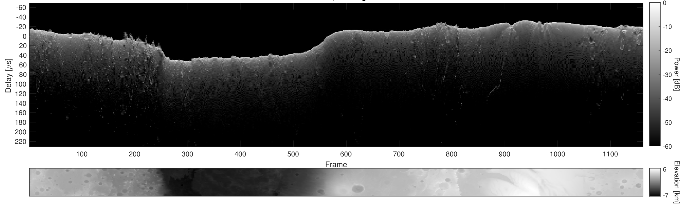
Orbit 11022, Cluttergram
