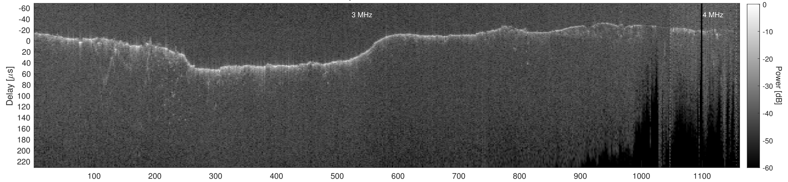
Orbit 11022, Cluttergram
