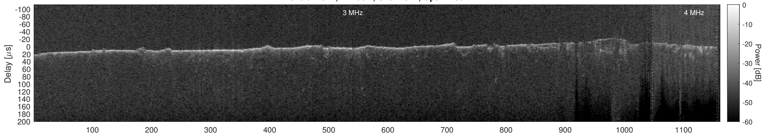
Orbit 11024, Cluttergram
