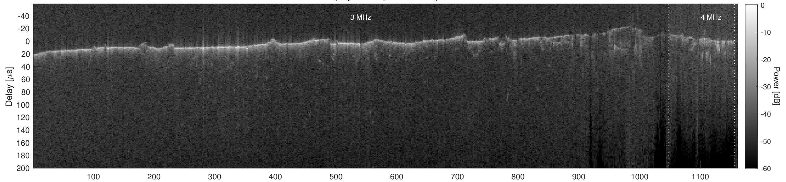
Orbit 11024, Cluttergram
