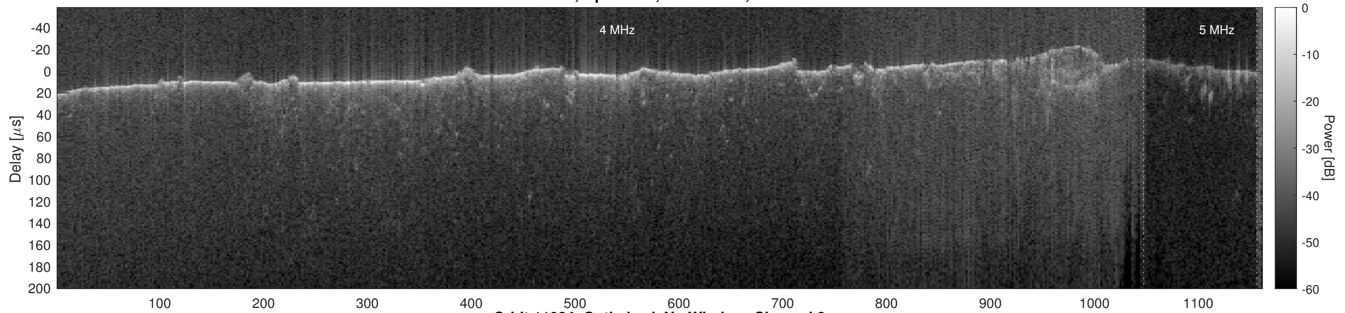
Orbit 11024, Optimized, No Window, Channel 2
