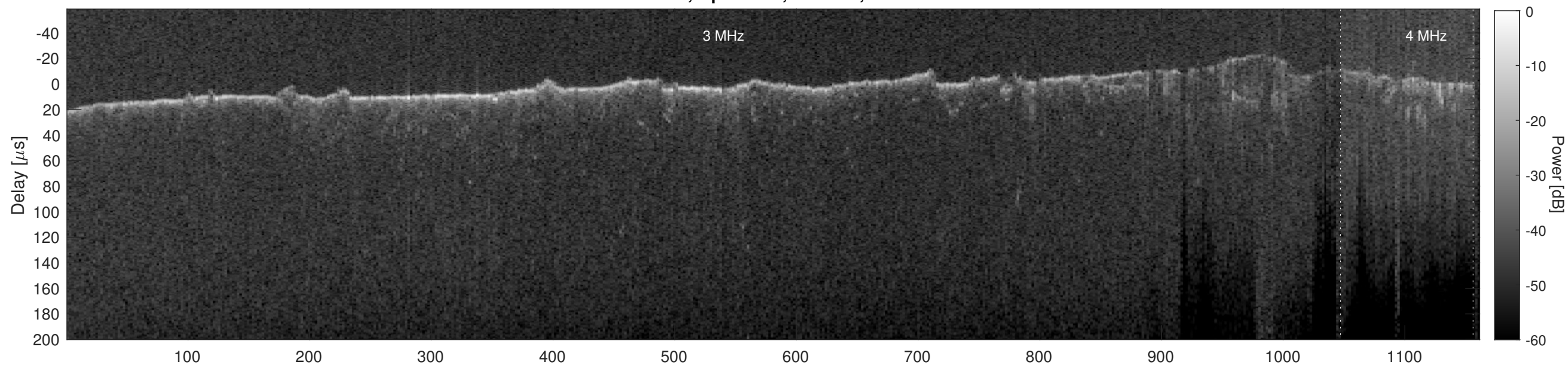
Orbit 11024, Cluttergram
