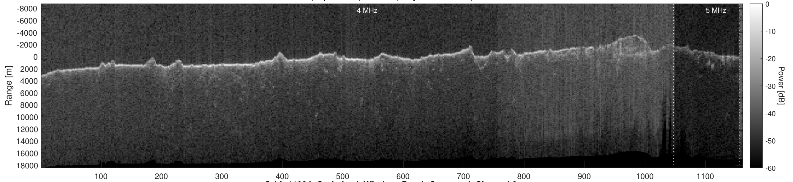
Orbit 11024, Optimized, Window, Depth-Corrected, Channel 2
