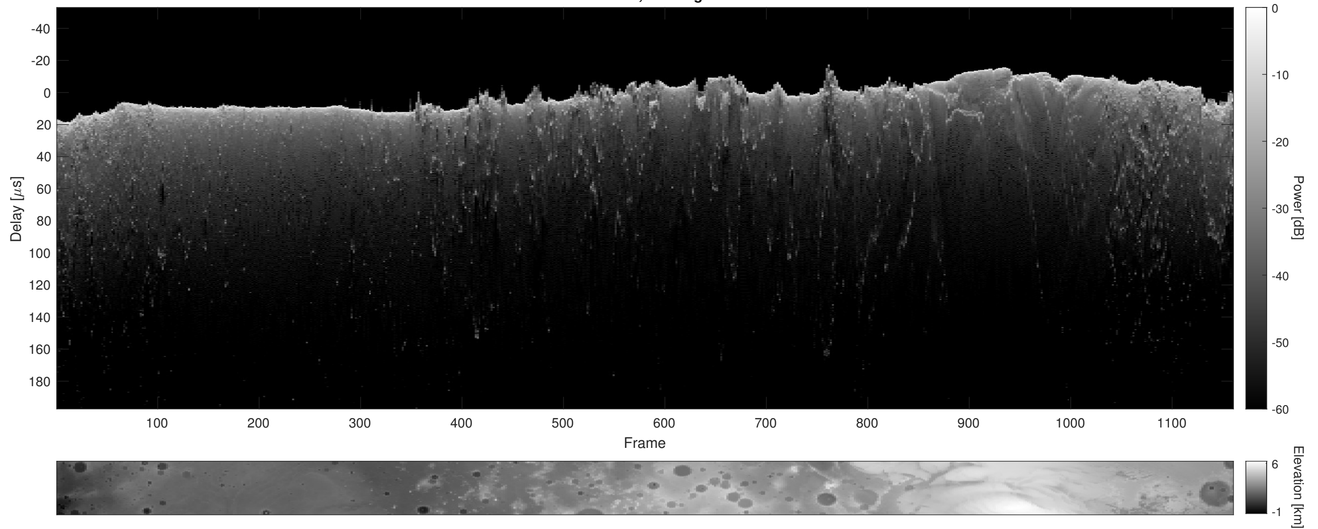
Orbit 11025, Cluttergram
