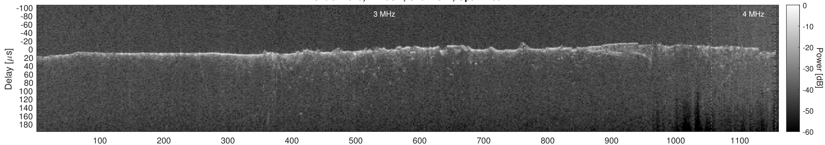
Orbit 11025, Cluttergram
