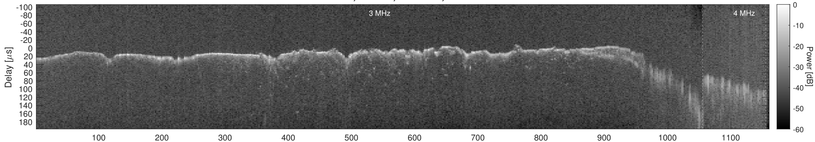
Orbit 11025, Window, Channel 2, Chapman
