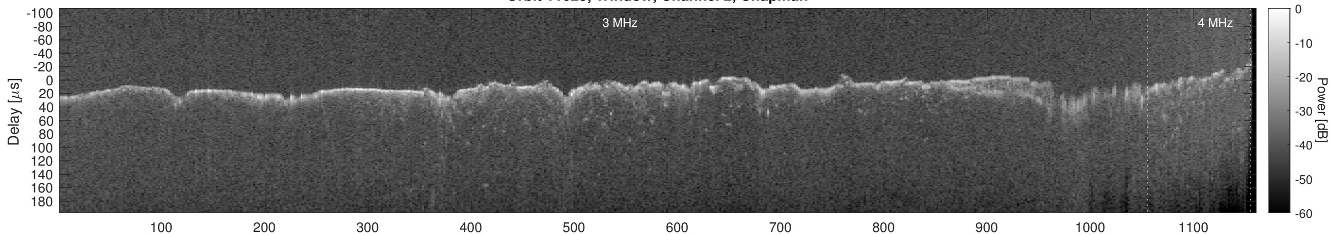
Orbit 11025, Window, Channel 2, Optimized
