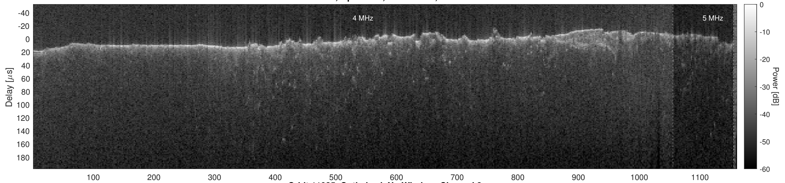
Orbit 11025, Optimized, No Window, Channel 2
