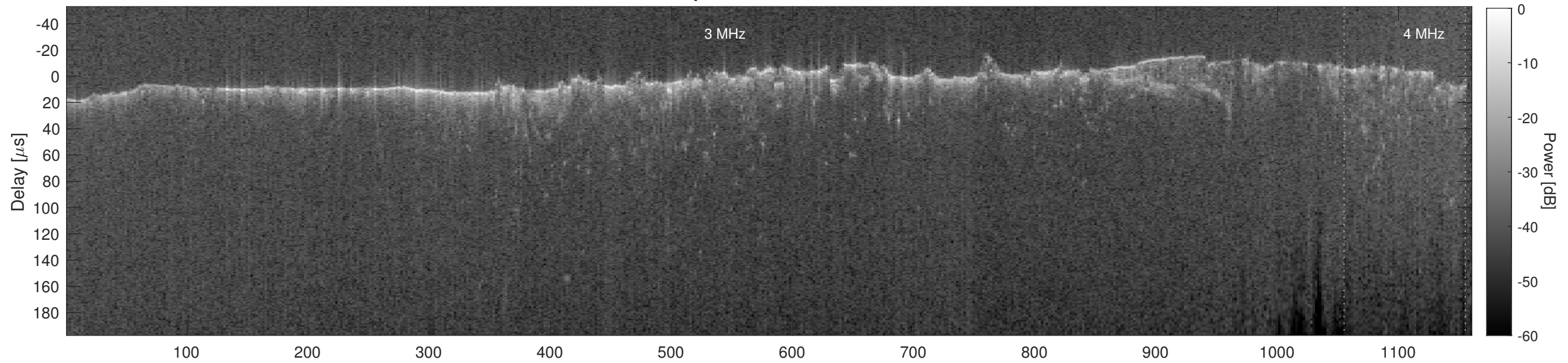
Orbit 11025, Cluttergram
