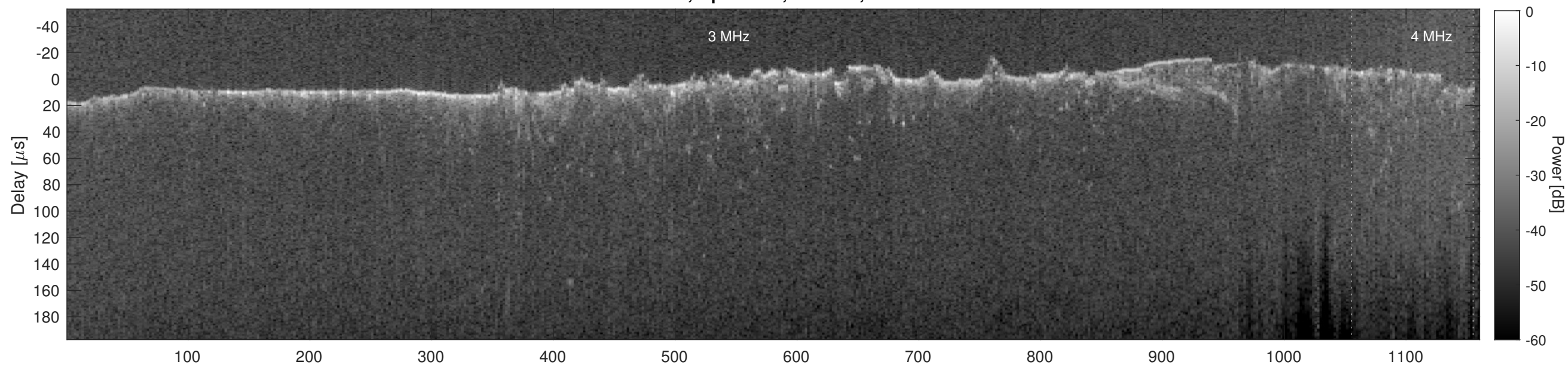
Orbit 11025, Cluttergram
