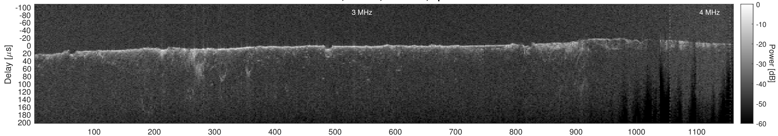
Orbit 11026, Cluttergram
