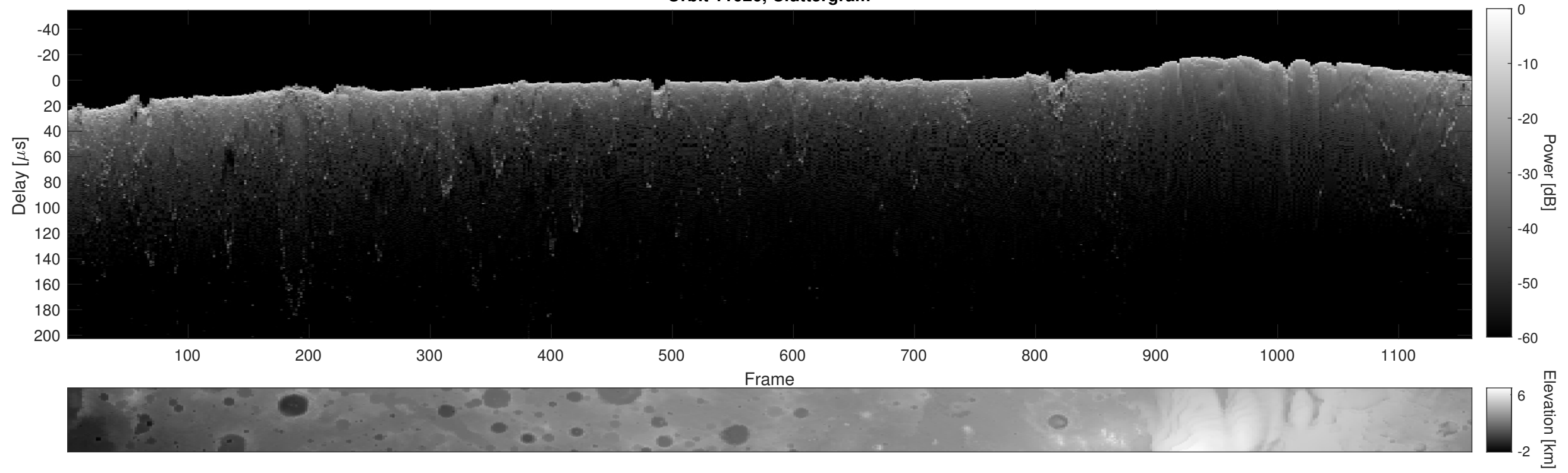
Orbit 11026, Cluttergram
