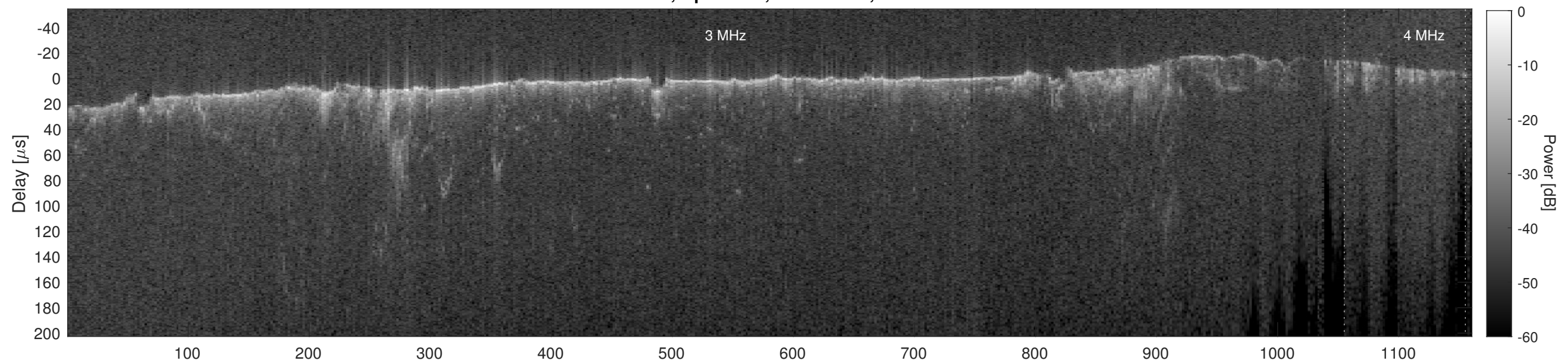
Orbit 11026, Cluttergram
