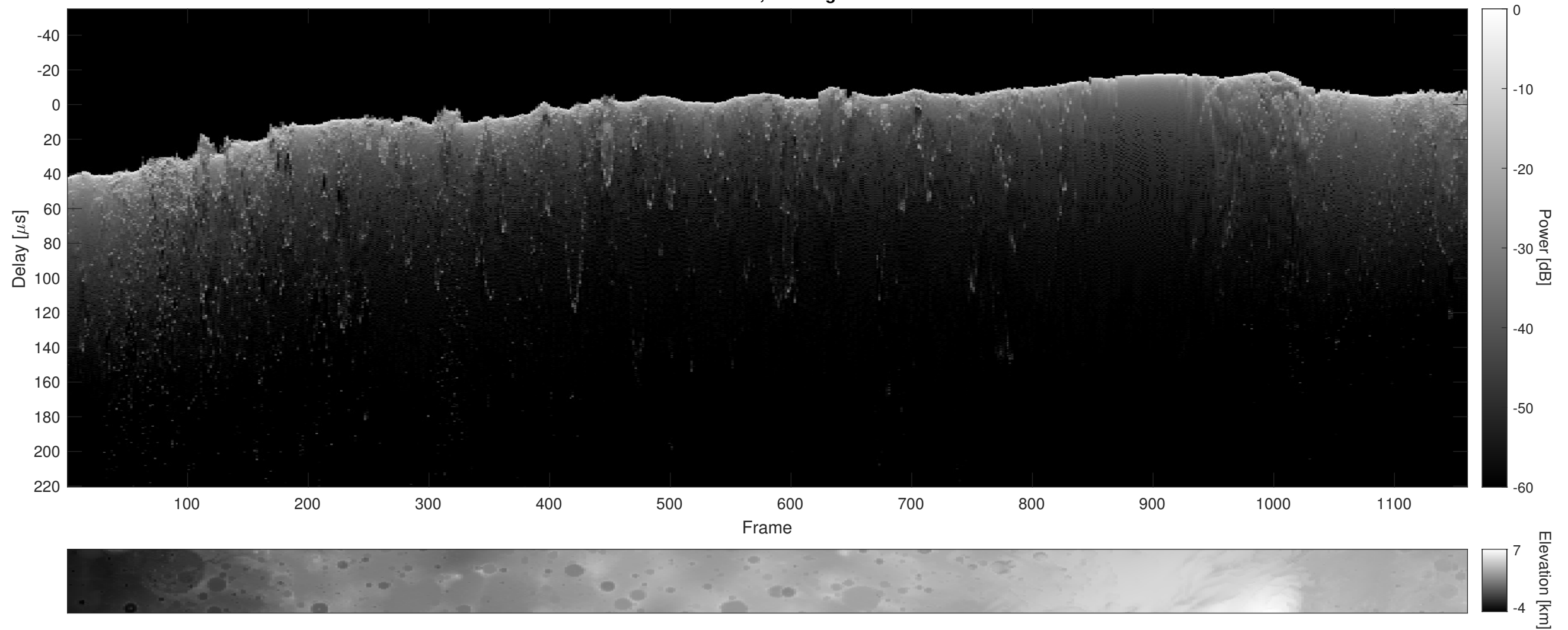
Orbit 11028, Cluttergram
