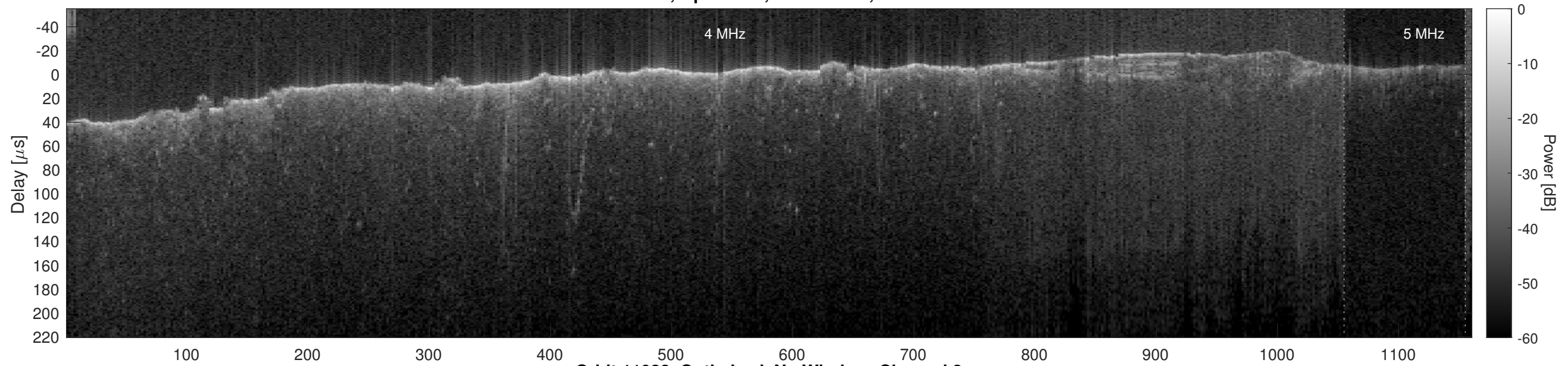
Orbit 11028, Optimized, No Window, Channel 2
