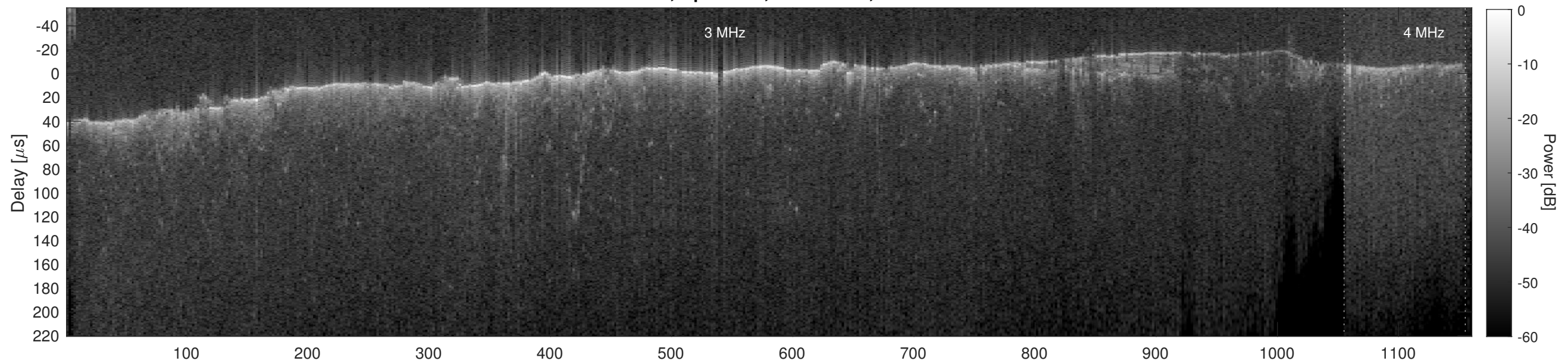
Orbit 11028, Cluttergram
