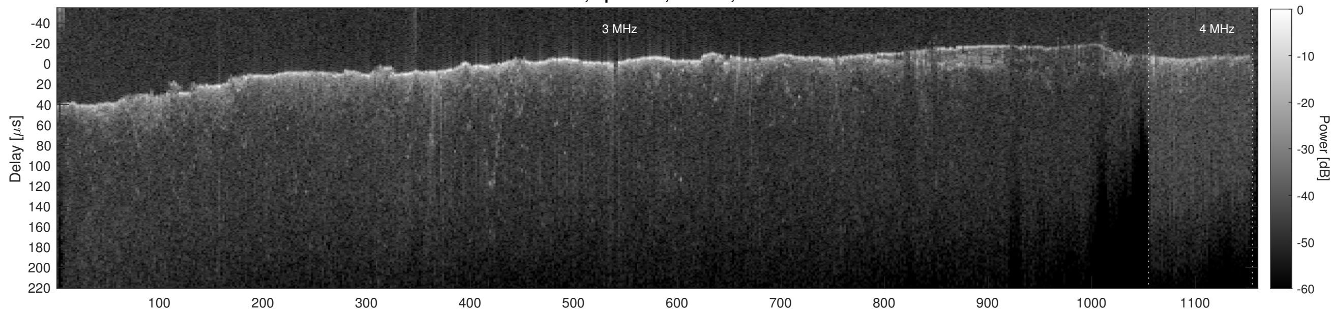
Orbit 11028, Cluttergram
