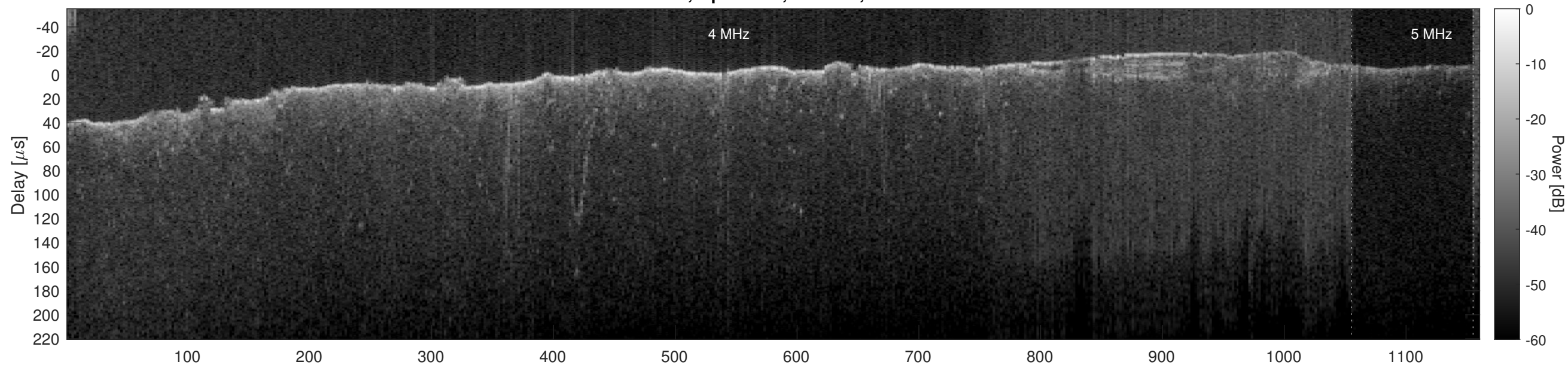
Orbit 11028, Optimized, Window, Channel 2
