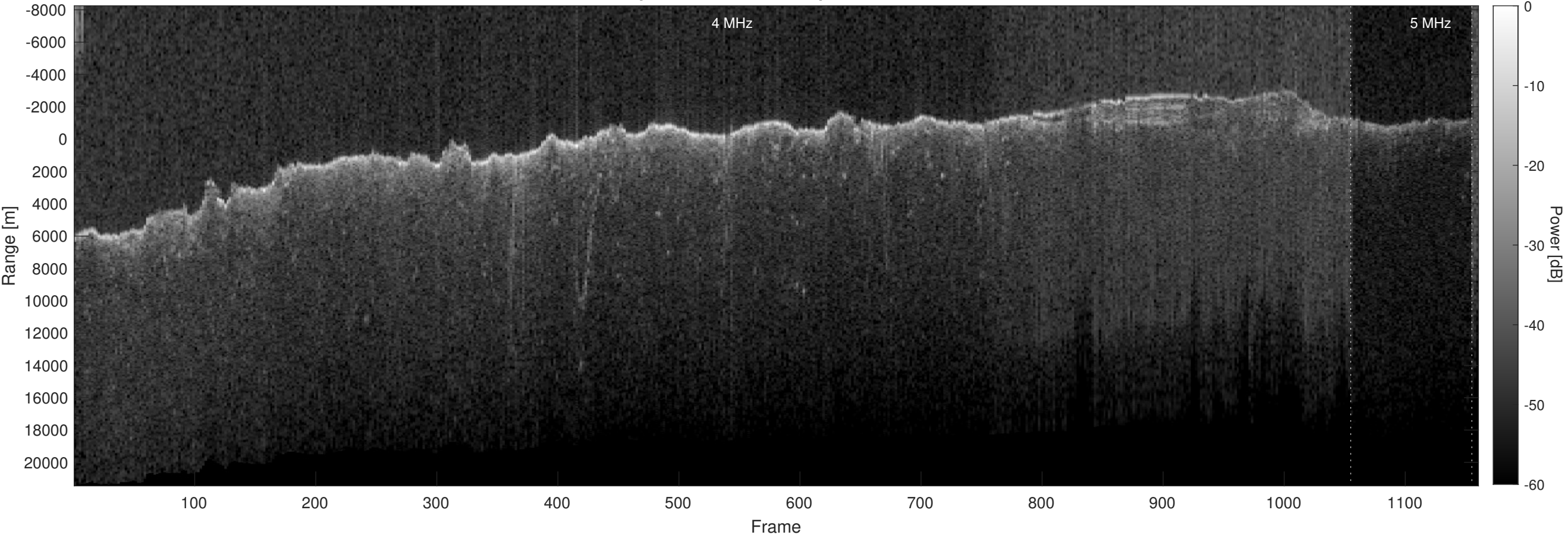
Orbit 11028, Optimized, Window, Depth-Corrected, Channel 2
