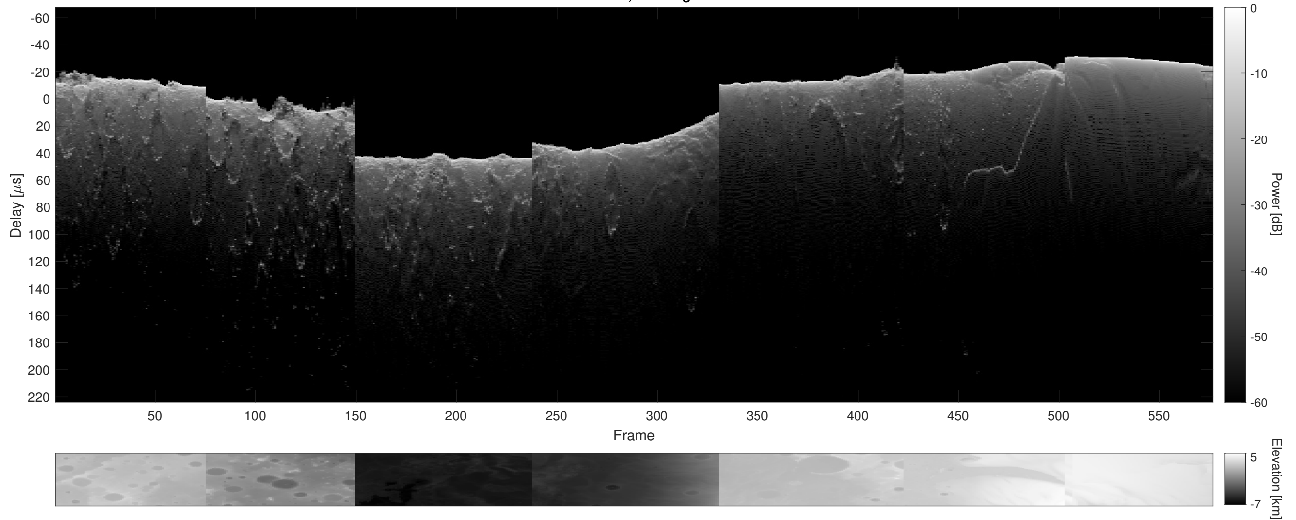
Orbit 11029, Cluttergram
