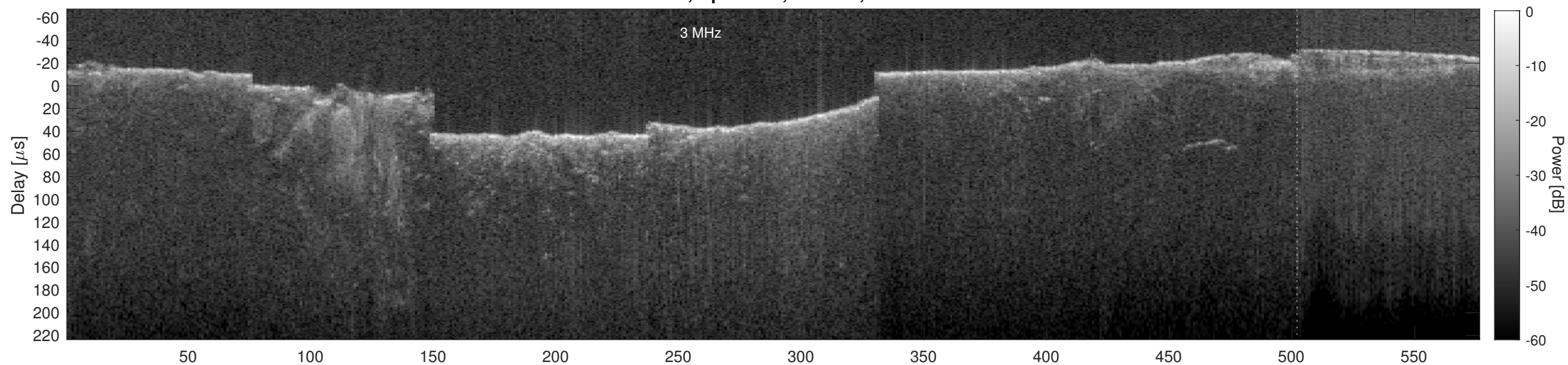
Orbit 11029, Cluttergram
