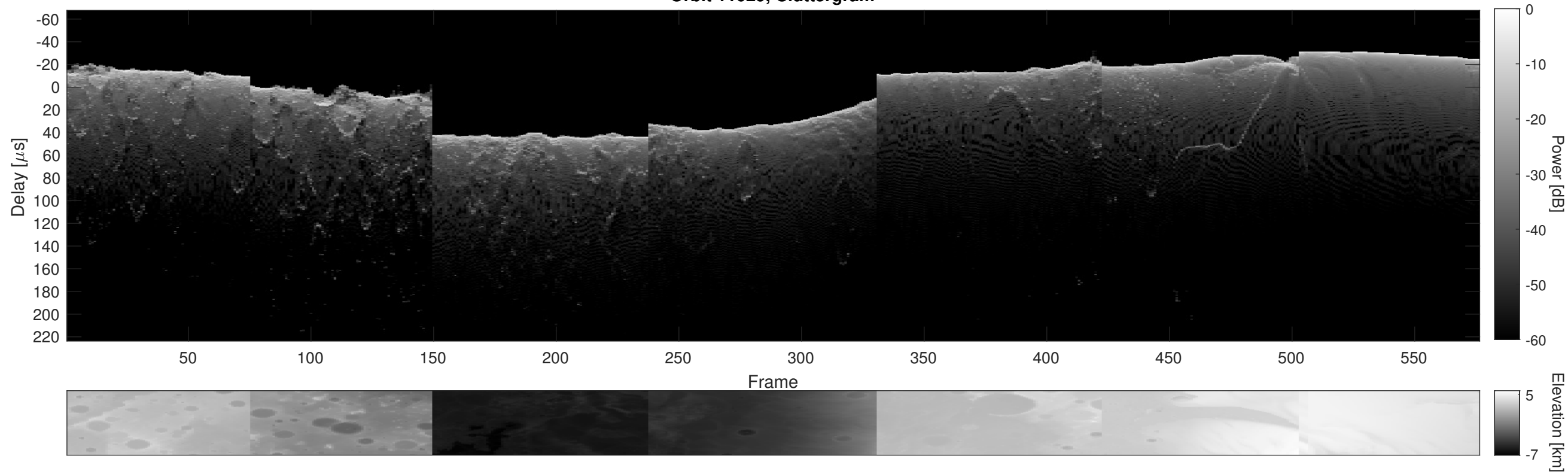
Orbit 11029, Cluttergram
