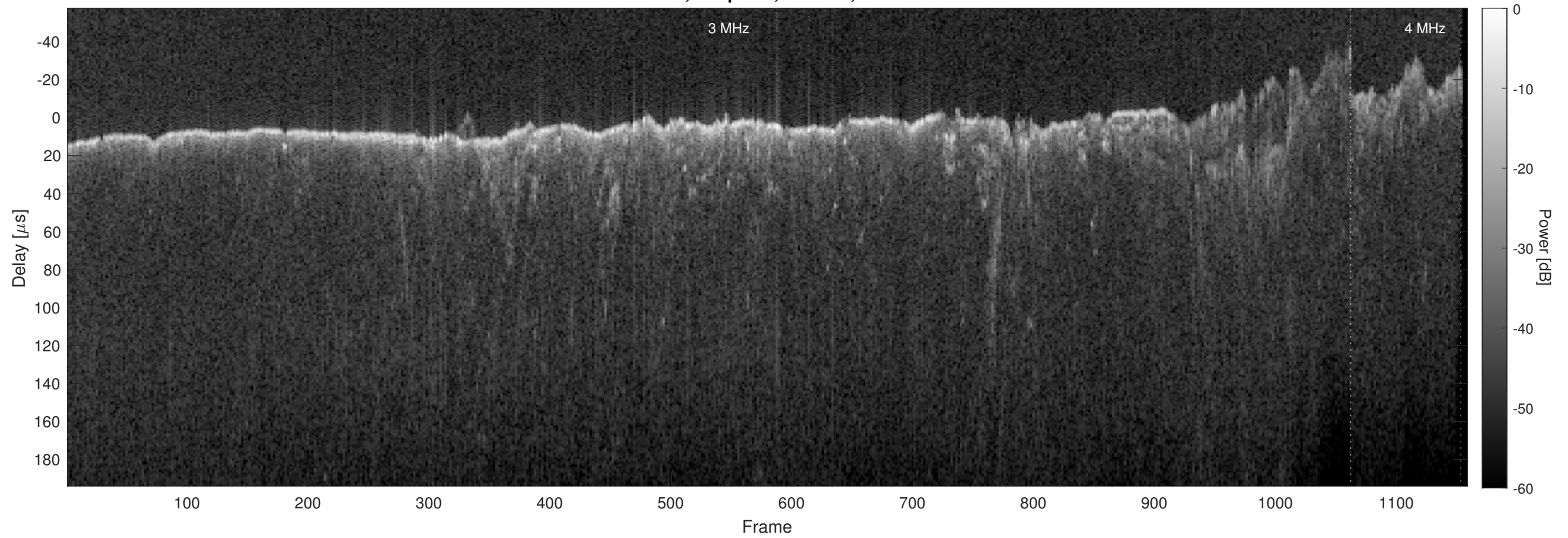
Orbit 11031, Chapman, Window, Channel 2
