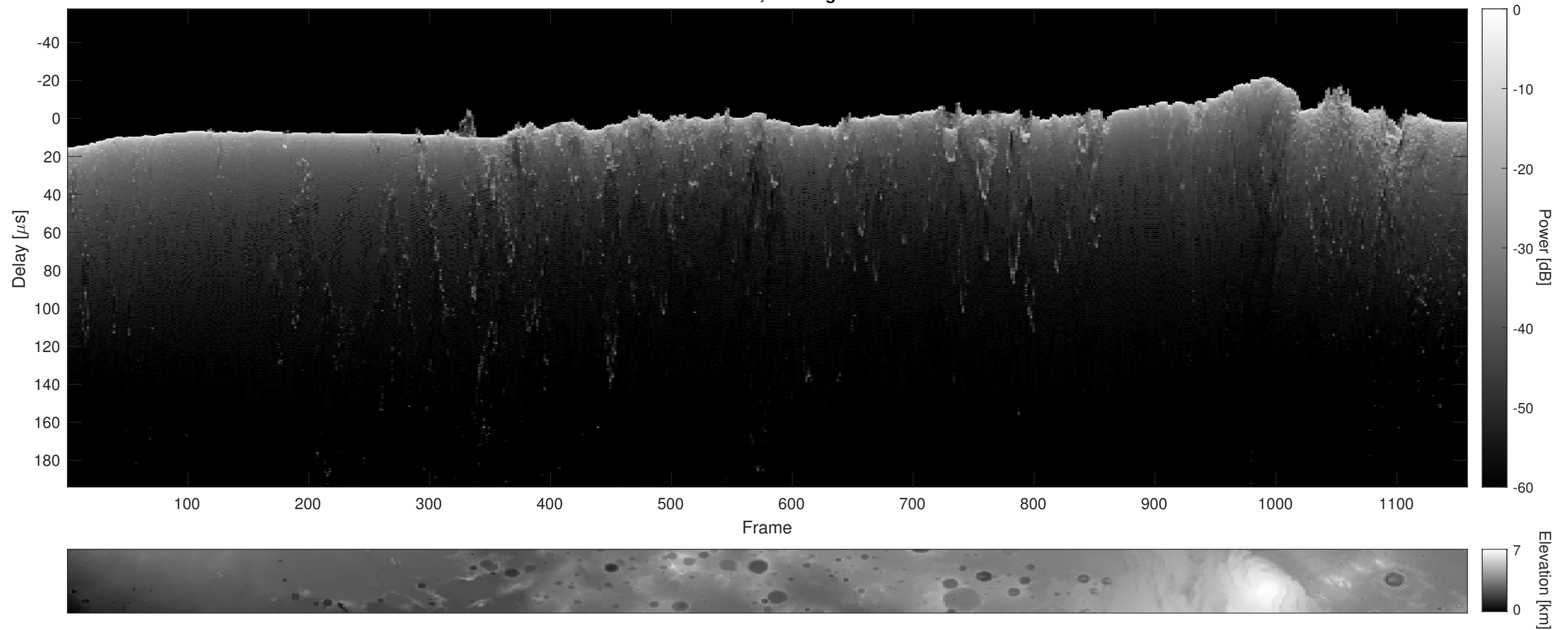
Orbit 11031, Cluttergram
