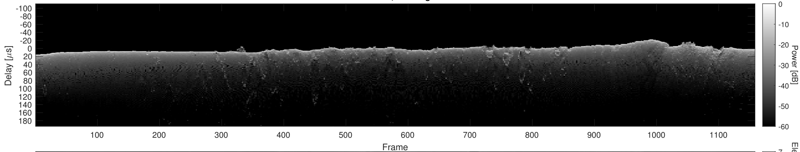
Orbit 11031, Cluttergram
