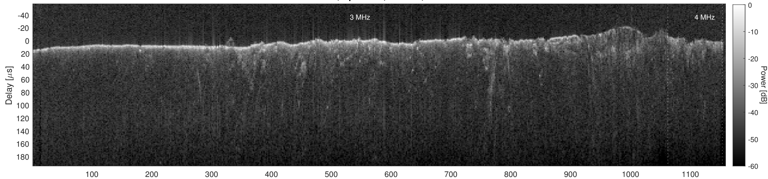
Orbit 11031, Cluttergram
