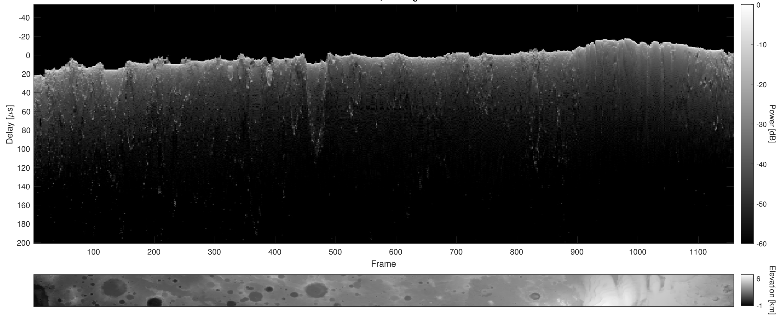
Orbit 11033, Cluttergram
