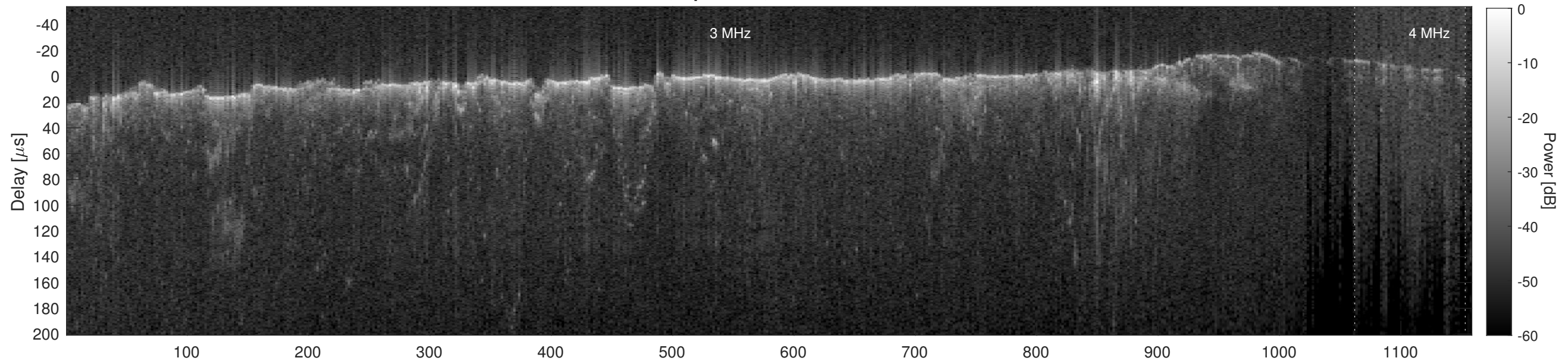
Orbit 11033, Cluttergram
