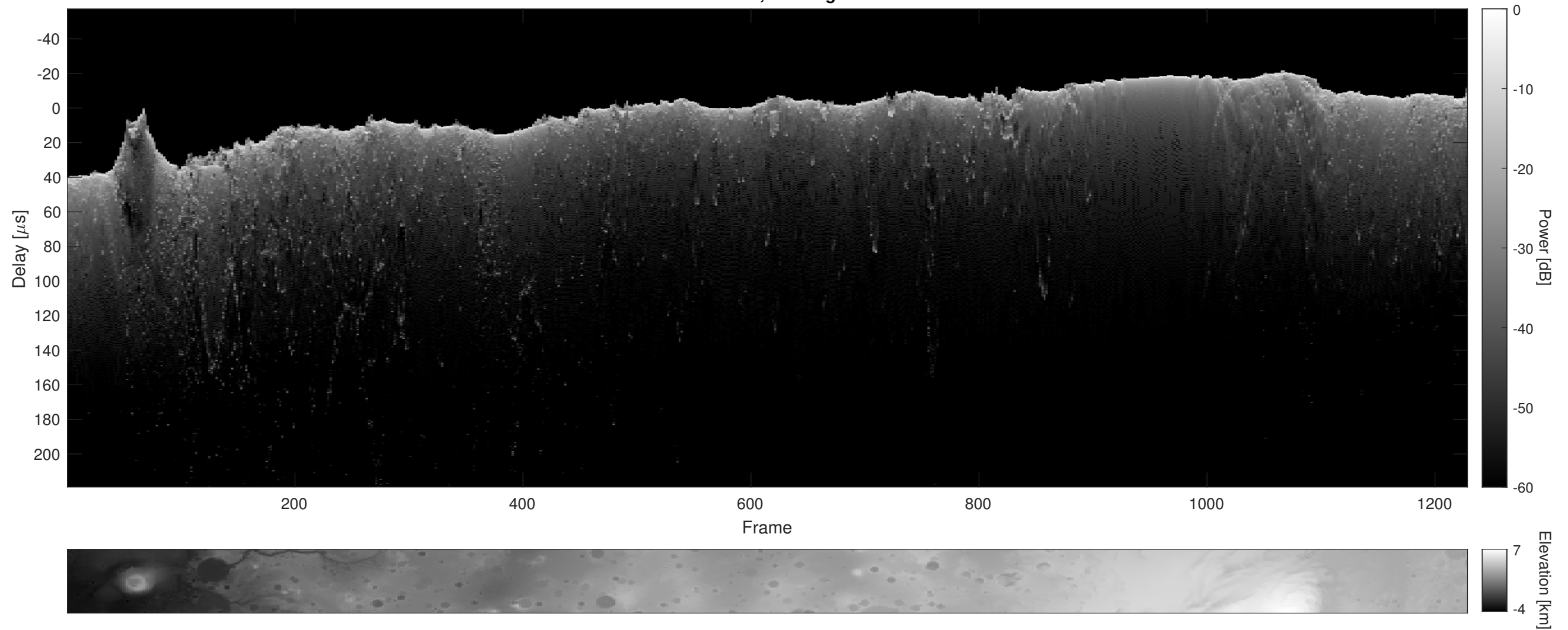
Orbit 11035, Cluttergram
