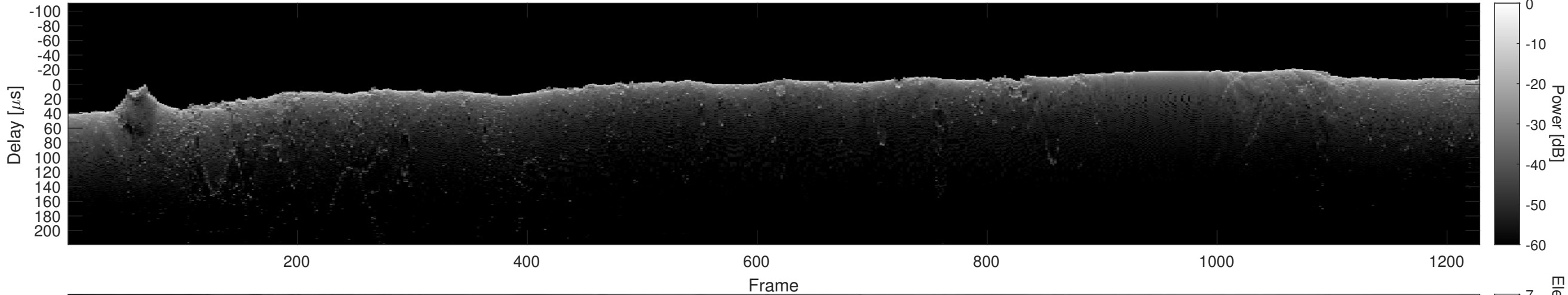
Orbit 11035, Cluttergram
