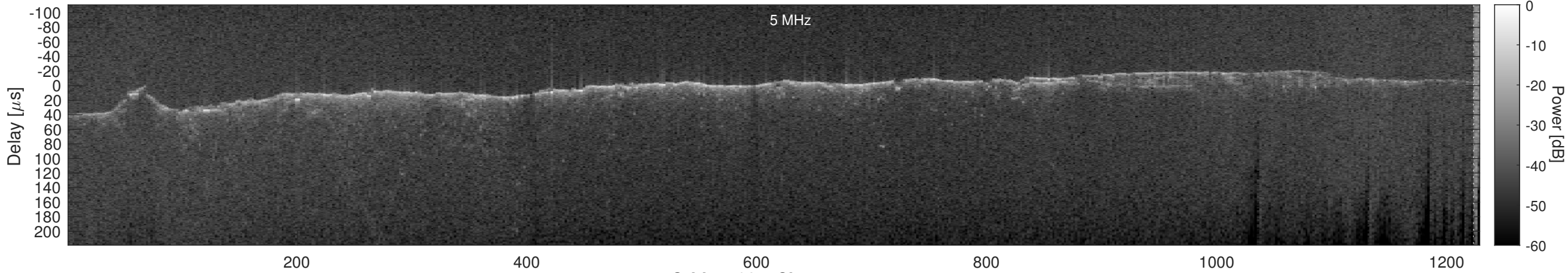
Orbit 11035, Cluttergram
