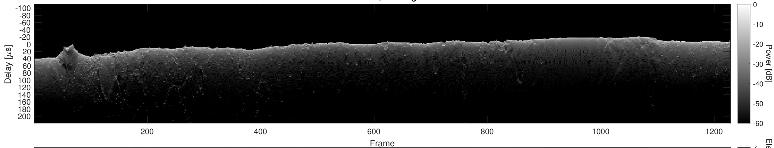
Orbit 11035, Cluttergram
