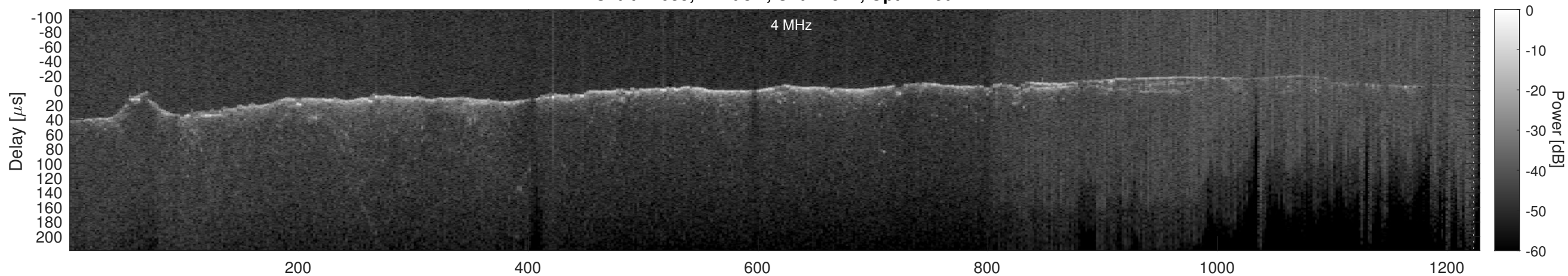
Orbit 11035, Cluttergram
