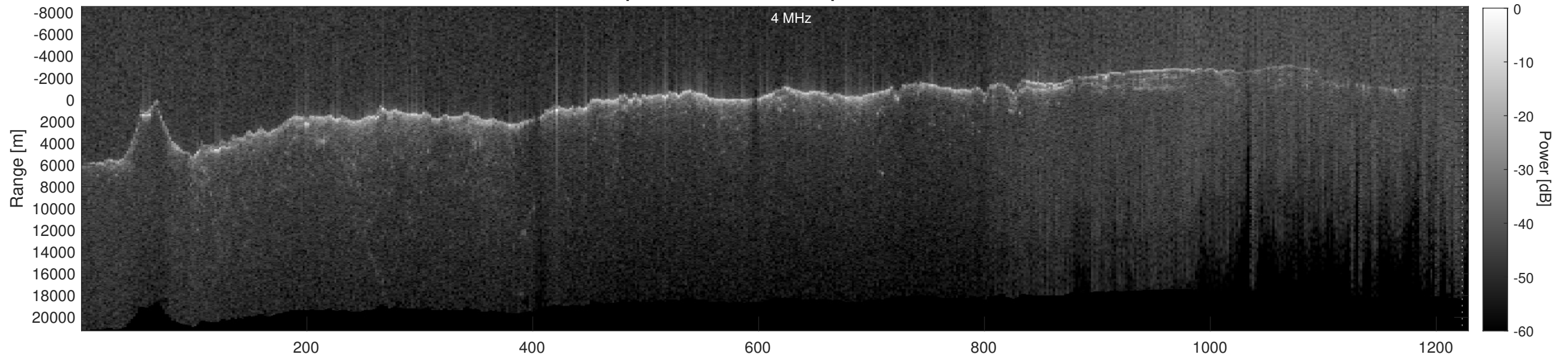
Orbit 11035, Depth-Corrected Cluttergram
