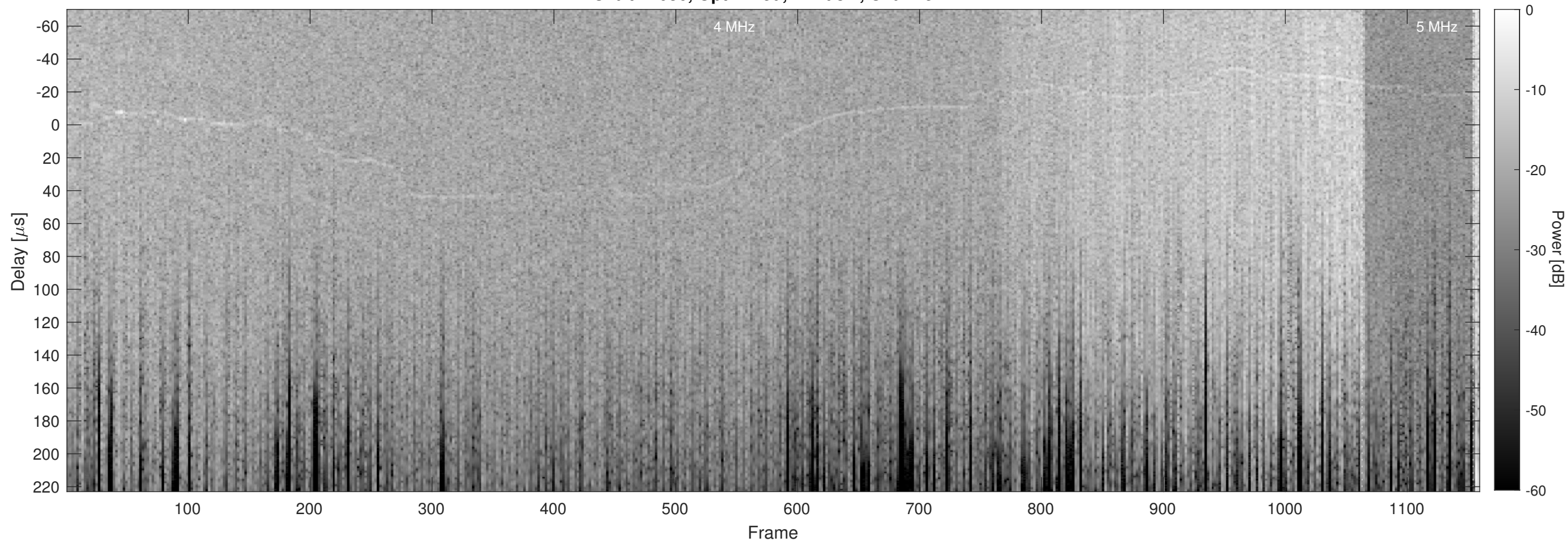
Orbit 11036, Optimized, Window, Channel 2
