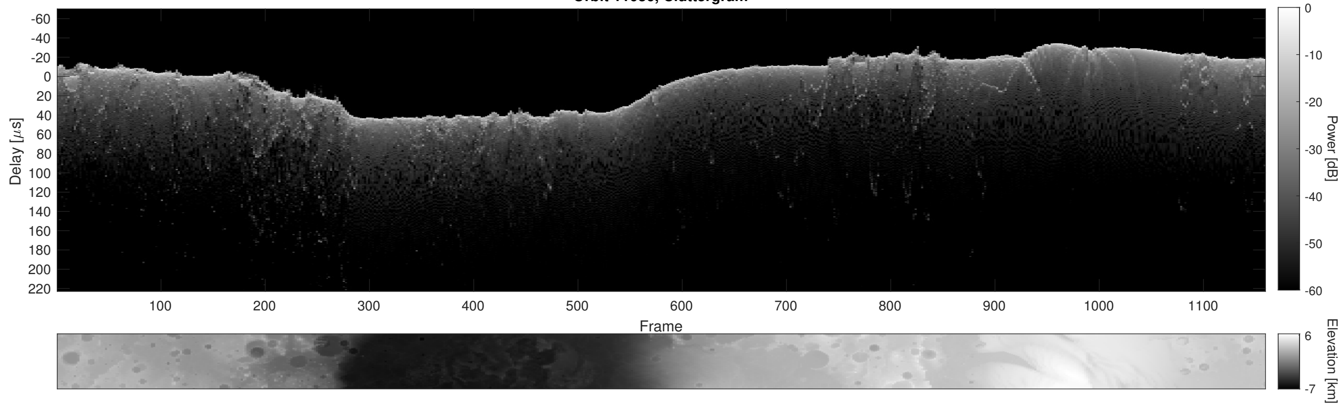
Orbit 11036, Cluttergram
