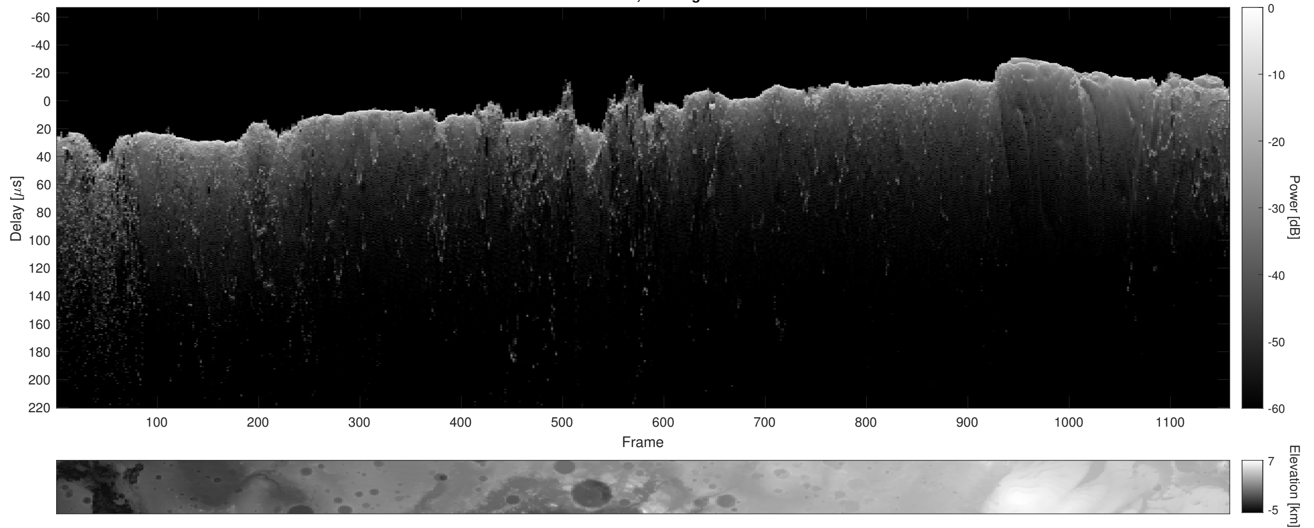
Orbit 11037, Cluttergram
