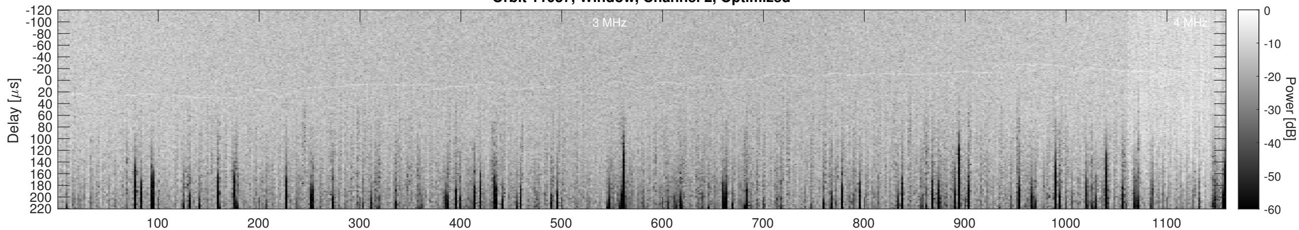
Orbit 11037, Cluttergram
