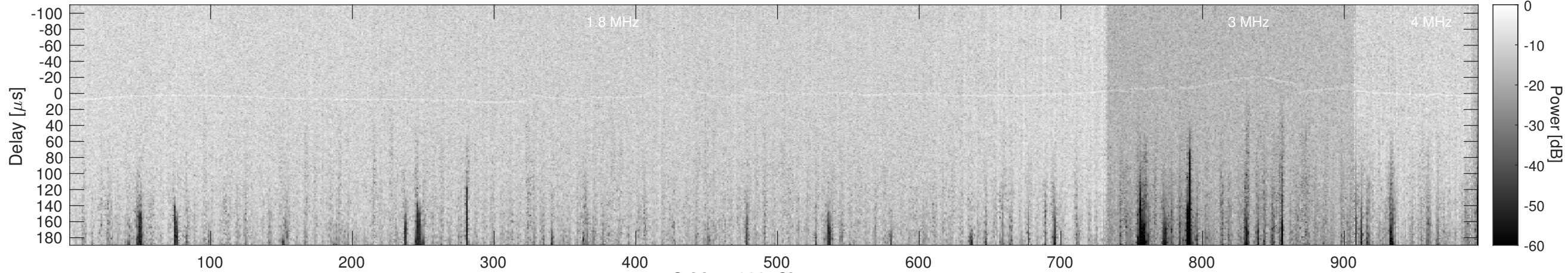
Orbit 11038, Cluttergram
