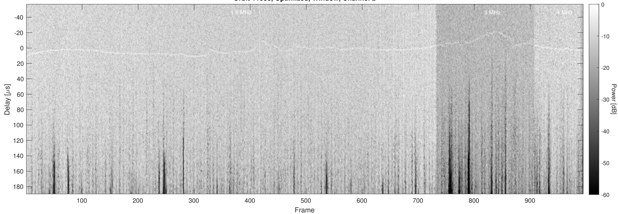
Orbit 11038, Optimized, Window, Channel 2
