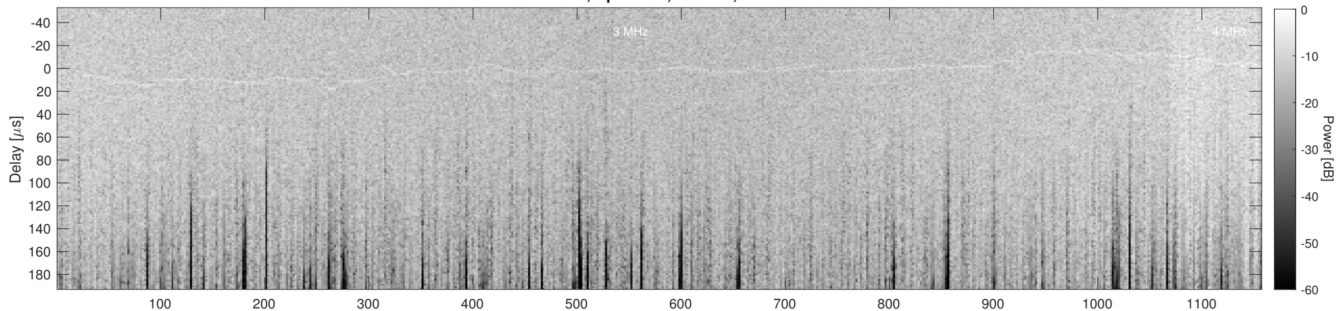
Orbit 11040, Cluttergram
