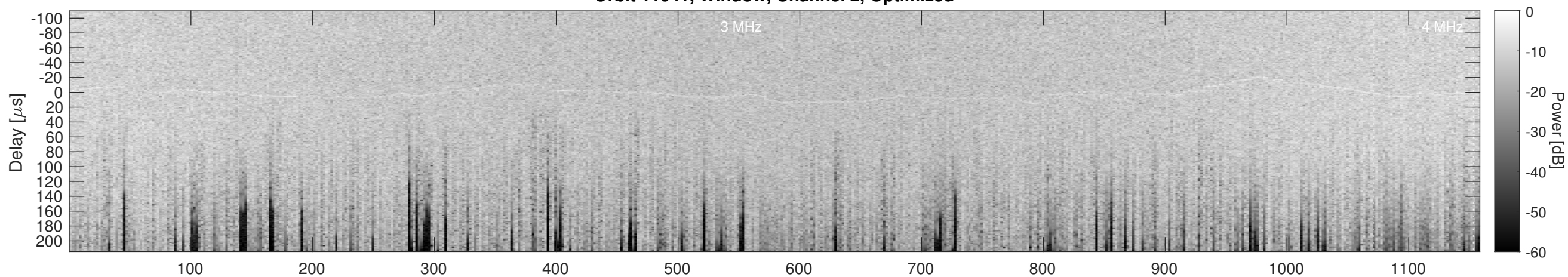
Orbit 11041, Cluttergram
