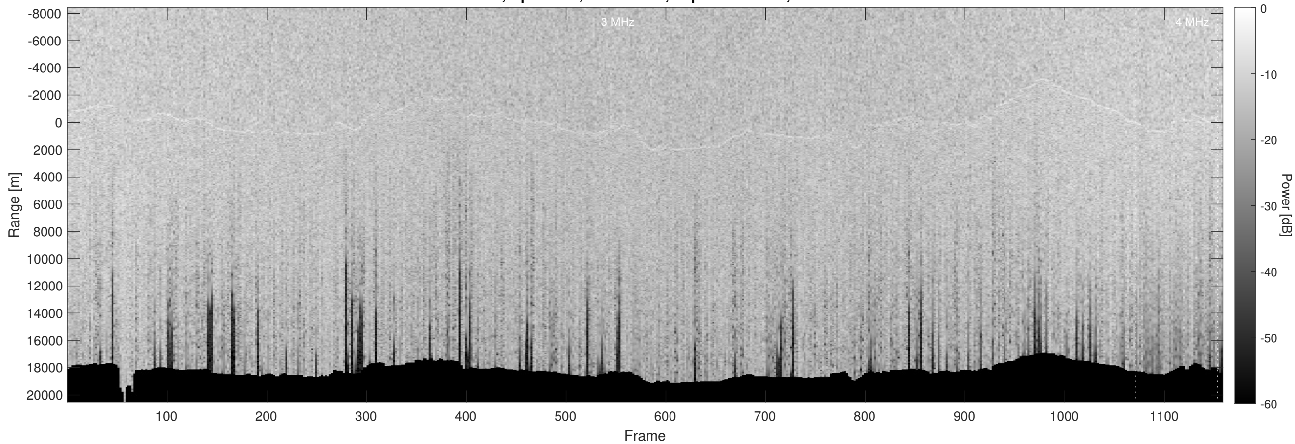
Orbit 11041, Optimized, No Window, Depth-Corrected, Channel 2
