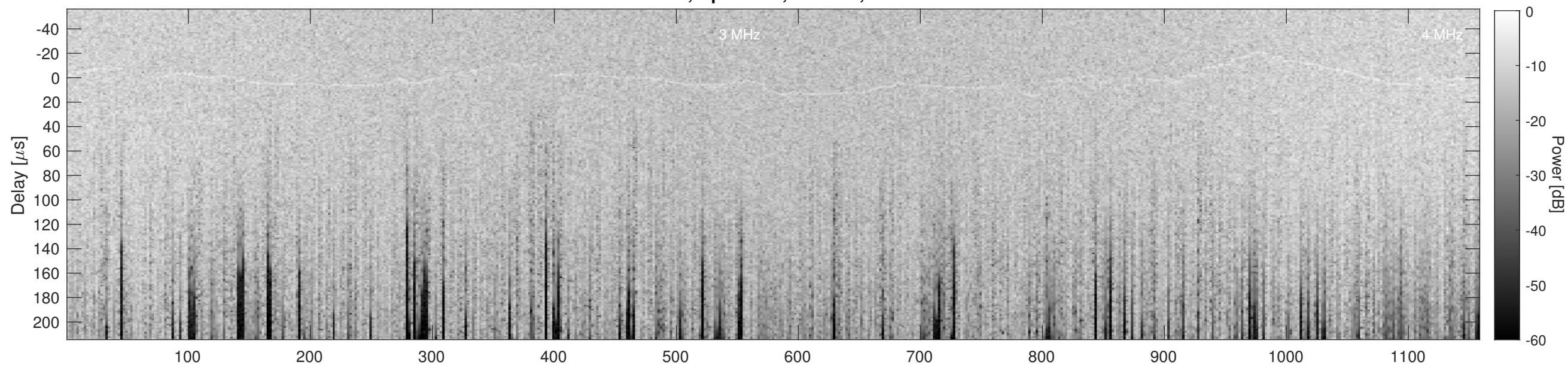
Orbit 11041, Cluttergram
