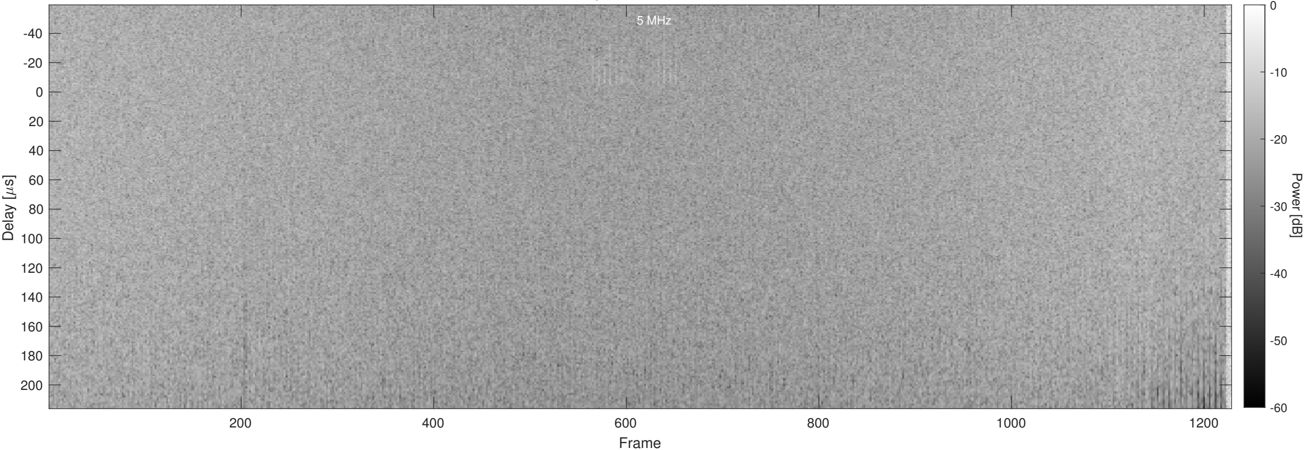
Orbit 11042, Chapman, No Window, Channel 2
