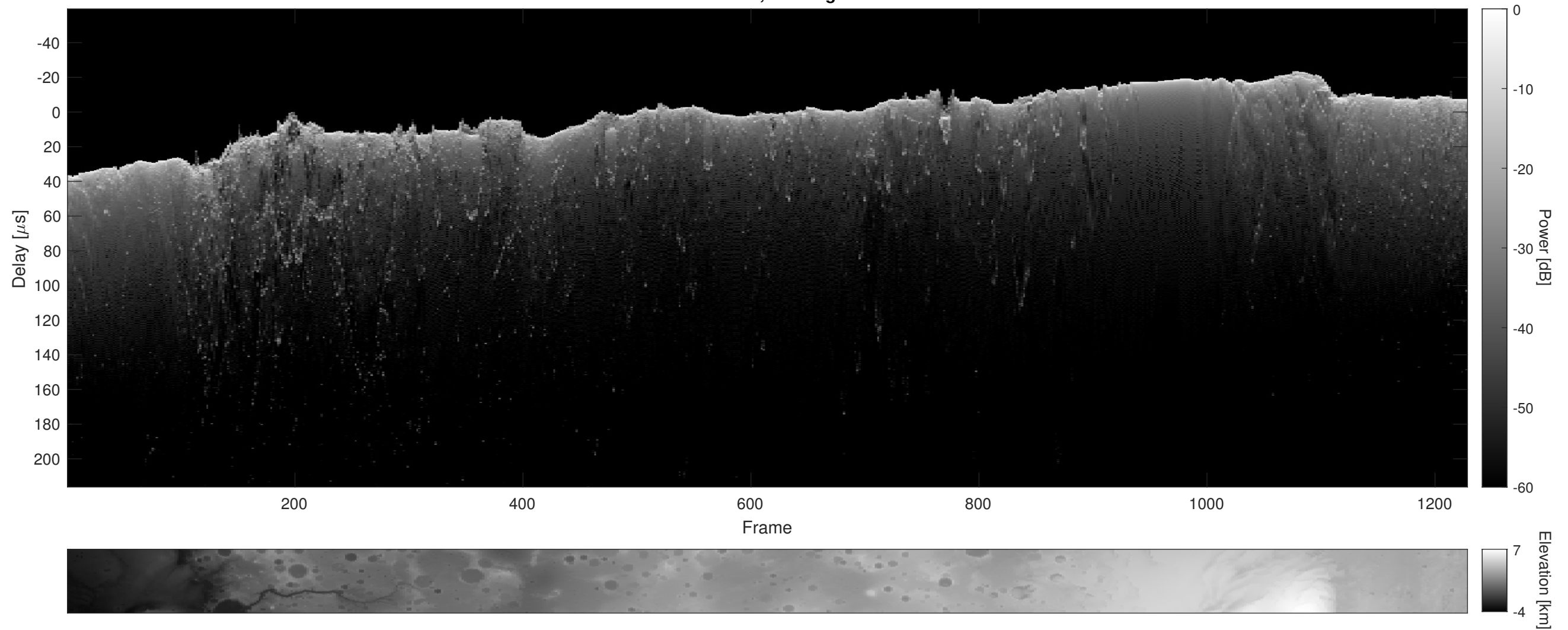
Orbit 11042, Cluttergram
