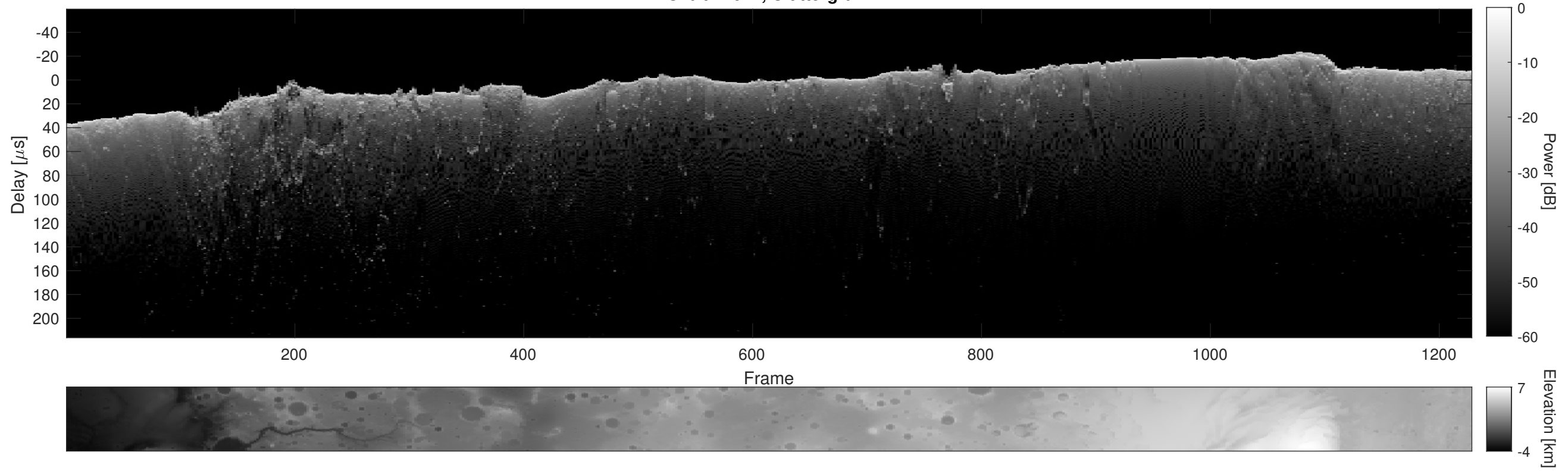
Orbit 11042, Cluttergram
