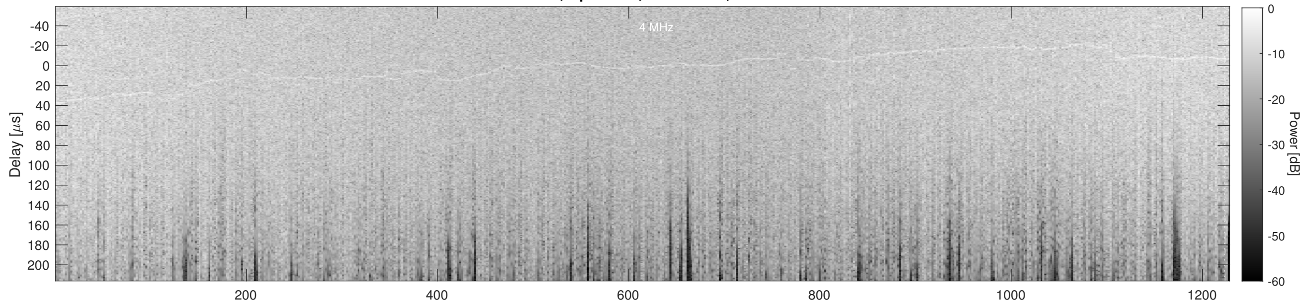
Orbit 11042, Cluttergram
