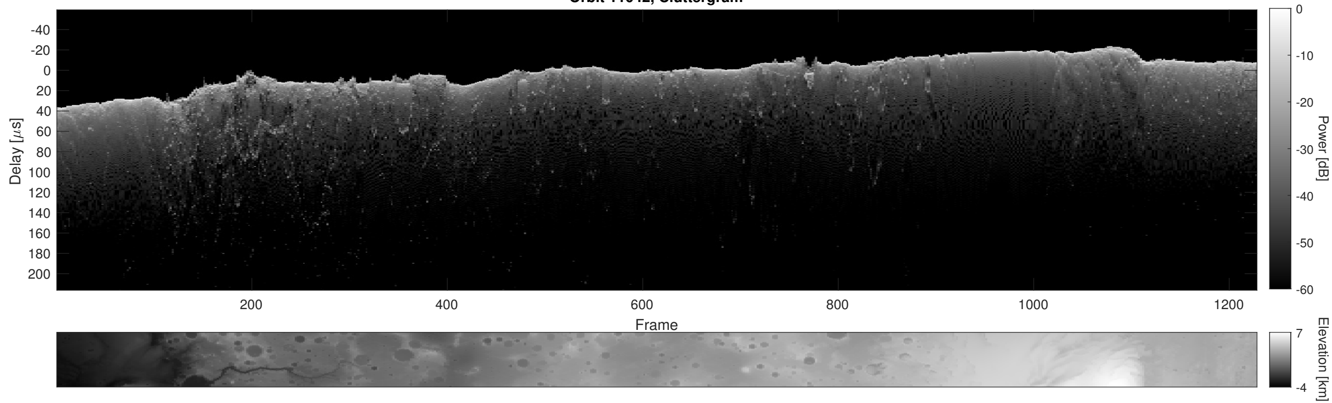
Orbit 11042, Cluttergram
