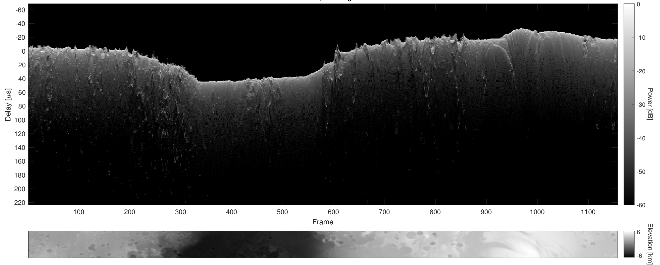
Orbit 11043, Cluttergram
