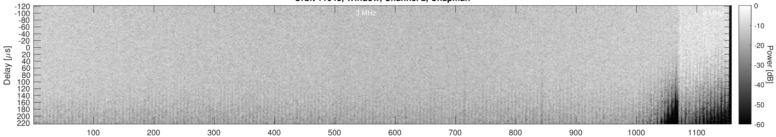
Orbit 11043, Window, Channel 2, Optimized
