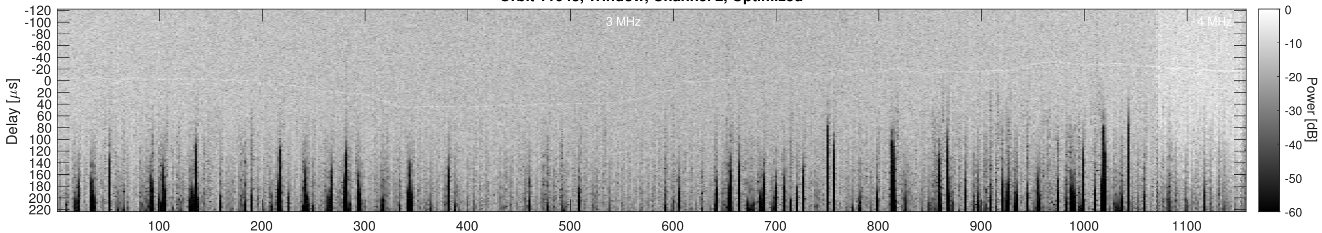
Orbit 11043, Cluttergram
