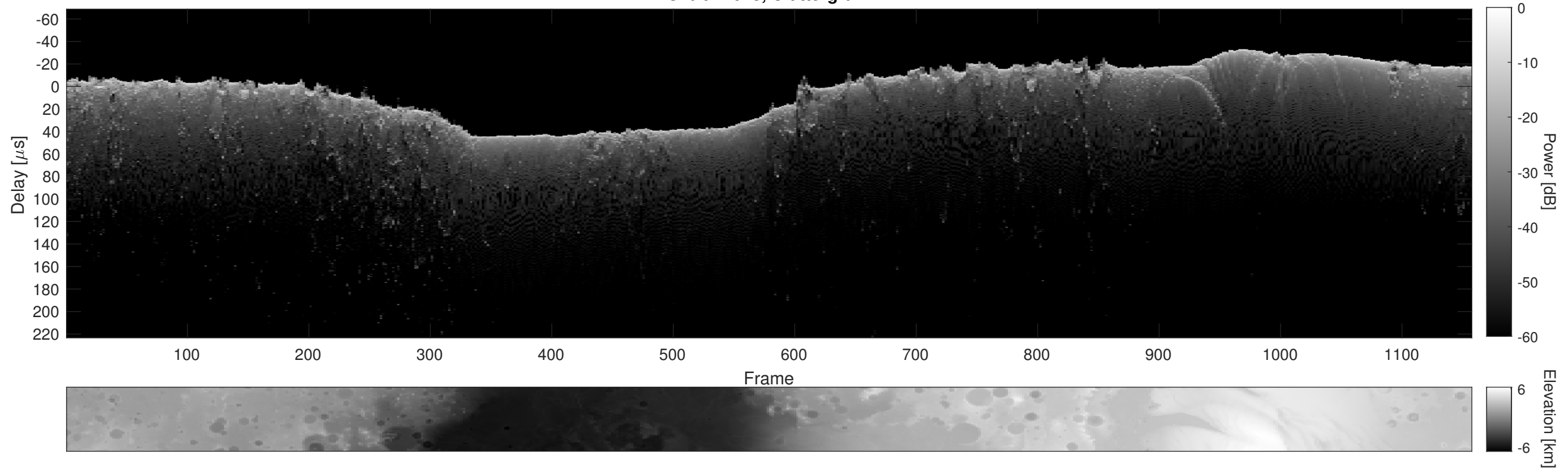
Orbit 11043, Cluttergram
