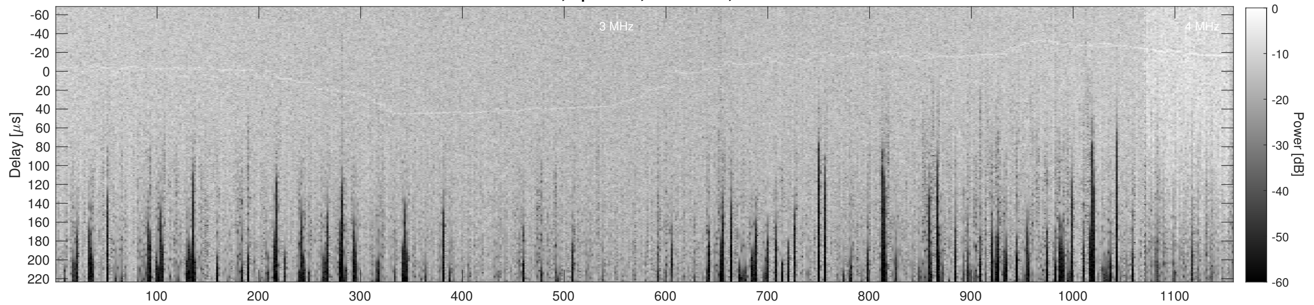
Orbit 11043, Cluttergram
