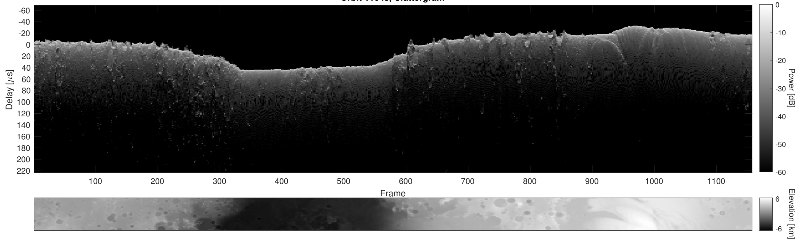
Orbit 11043, Cluttergram
