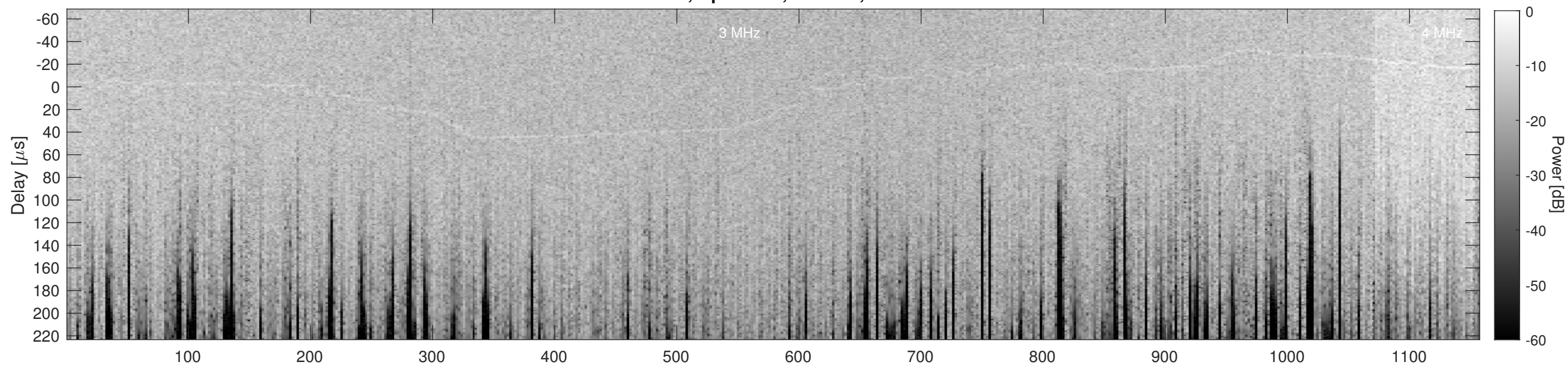
Orbit 11043, Cluttergram
