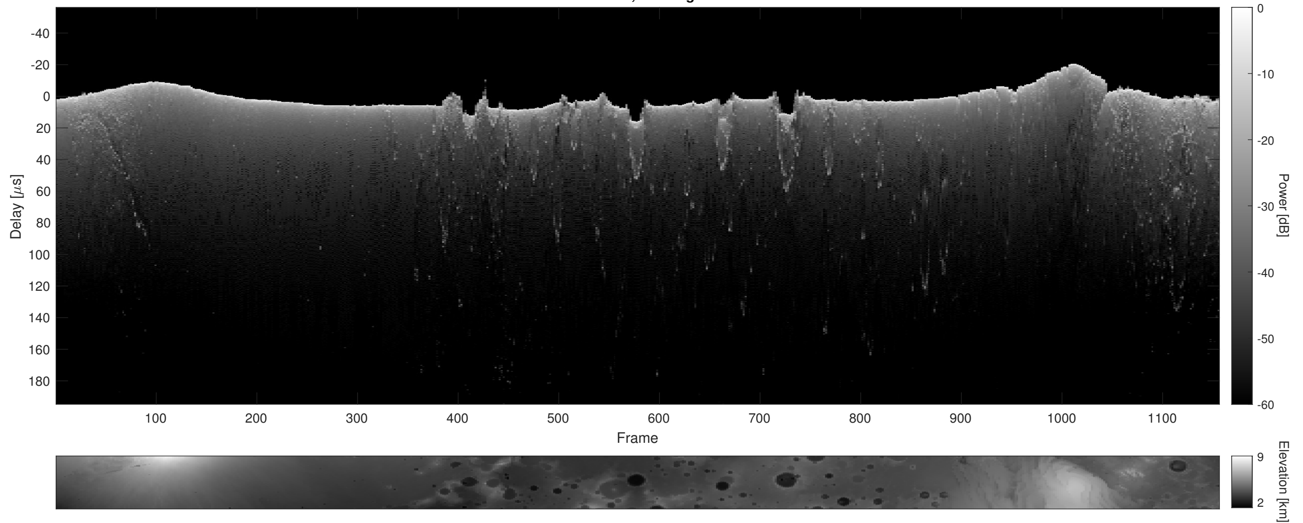
Orbit 11045, Cluttergram
